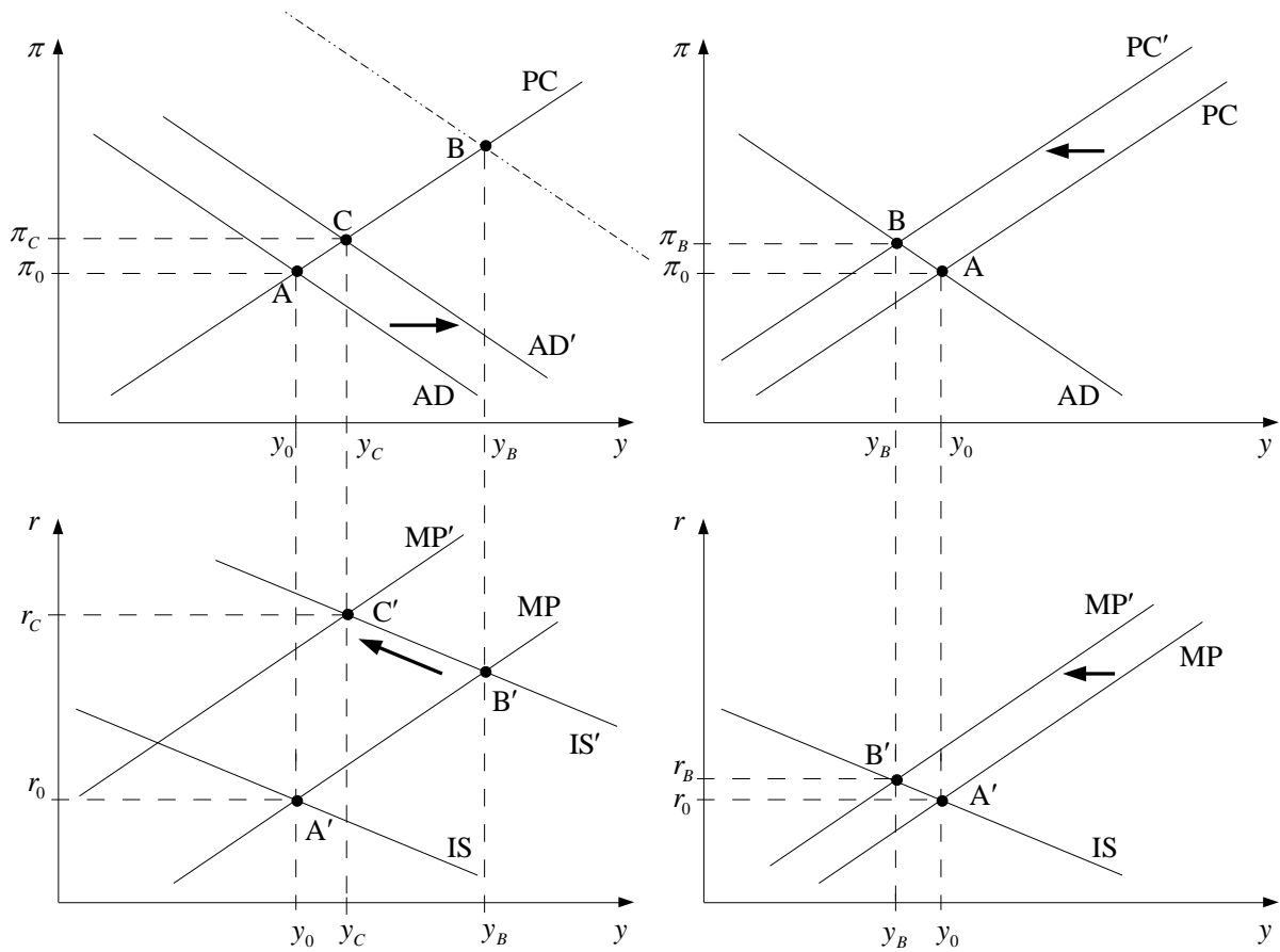
Figure 1: Demand shock
